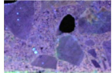
Dyed water penetration in Pavix treated concrete (<0.4 mm)
